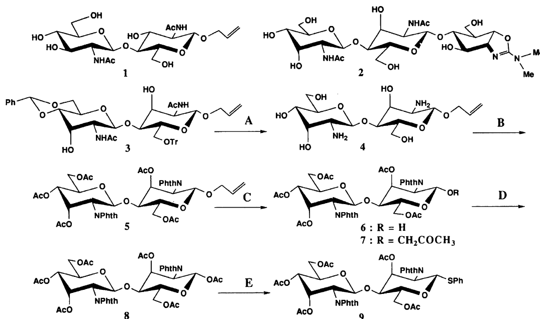
Scheme 1. Conditions: (A) i) 80% AcOH, 65 °C, ii) 1 M NaOH, 110 °C. (B) i) phthalic anhydride, Et 3 N, MeOH, ii) Ac 2 O, 4-dimethylaminopyridine, pyridine, RT. (C) PdCl 2 , NaOAc, aq AcOH, 50 °C. (D) NaOAc, Ac 2 O, 70 °C. (E) ZnI 2 , phenylthiotrimethylsilane, 1,2-dichloroethane, RT.
